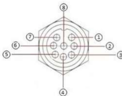
Figura 2: Conector TDL 5.0
