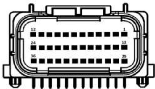
Figura 2: Conector CB 1204
