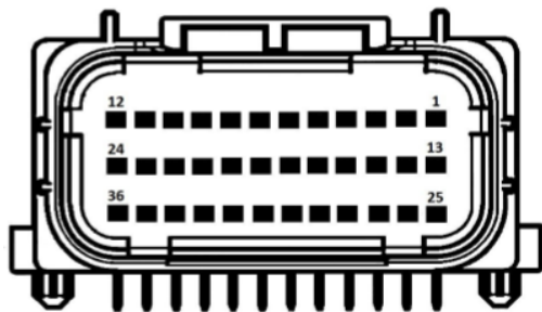
Figura 2: Conector CB 1204
